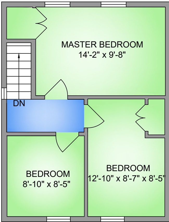
LOWER FLOOR 441 SQ. FT. 8' CEILING HEIGHT
