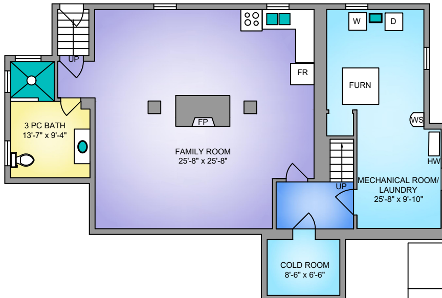
LOWER FLOOR 954 SQ. FT.
